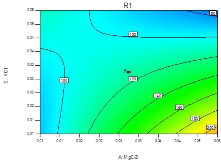
Fig. 3. Contour plot of effect of MgCl 2 and KCl on ALP production.
