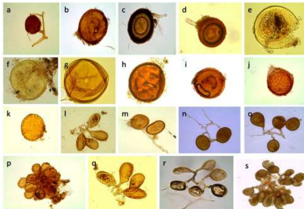
Figure 4. Some of the AMF spores isolated from Citrus rhizosphere soils; (a-d) Glomus spp., (e-k) Acaulospora spp., (l-s) Sporocarps.
