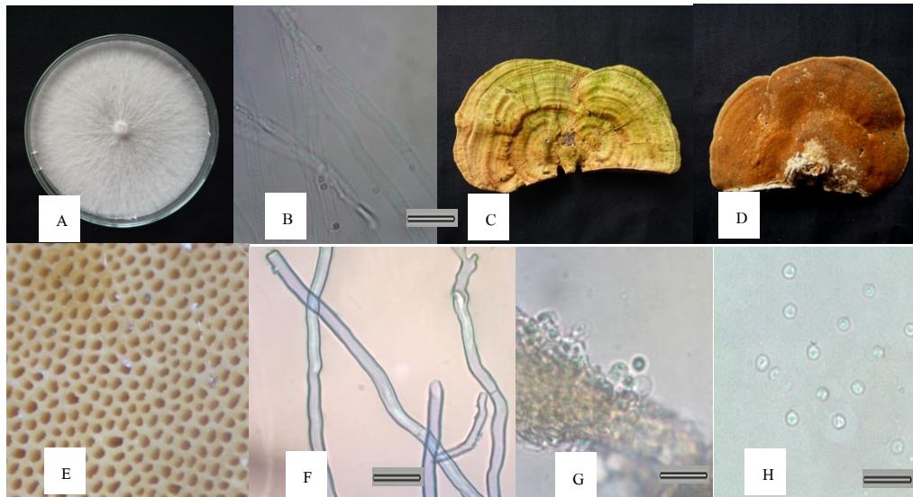
Fig. 1. The characteristic of Rigidoporus microporus SND04.
